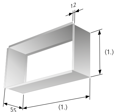
Figure 3. Fixing frame FHB. (1.) Nom. -3 mm.
