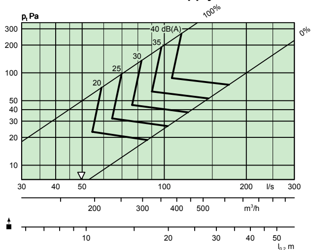
ALG 500-100 + TRG-B Ø200, Supply air
