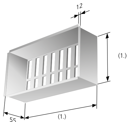
Figure 4. Fixing frame with sliding damper FHA. (1.) Nom. -3 mm.
