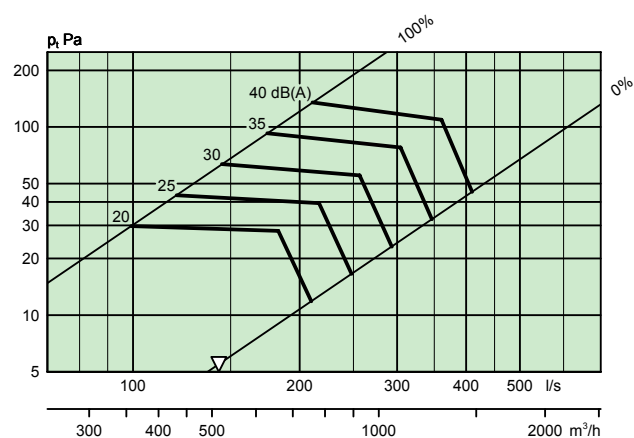
ALG 600-200 + TRG-B Ø315, Extract air
