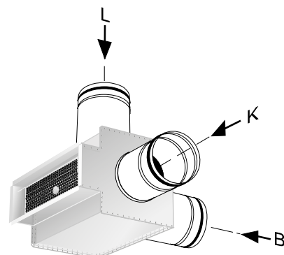
Figure 4. Fixing frame with sliding damper FHA. (1.) Nom. -3 mm.
