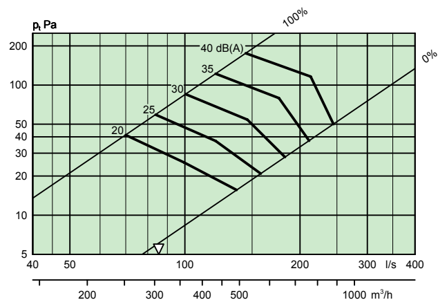
ALG 500-150 + TRG-B Ø250, Extract air
