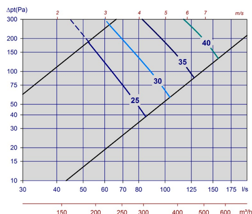
Diagram 2, Tellus-LÖV VAV-H/L Ø160, Max. spalt.
