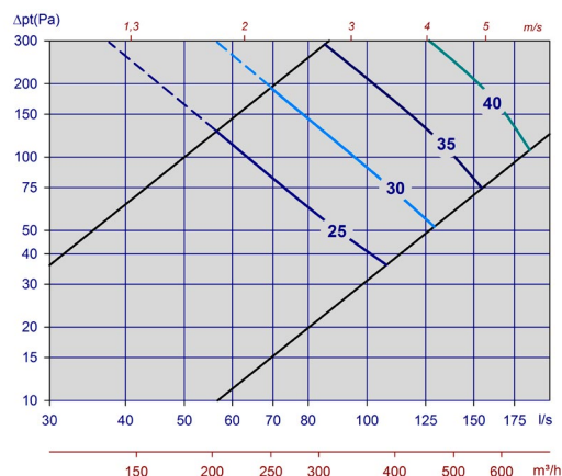
Diagram 3, Tellus-LÖV VAV-H/L Ø200 Max. spalt.
