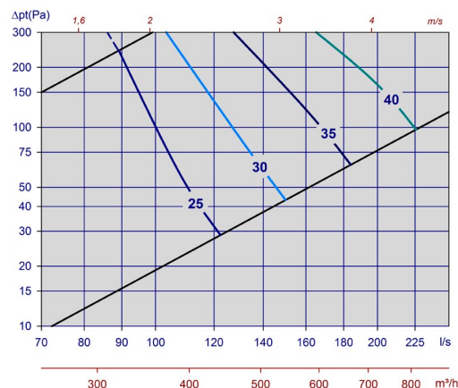
Diagram 4, Tellus-LÖV VAV-H/L Ø250 Max. spalt.
