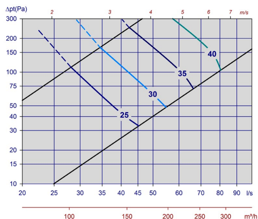
Diagram 1, Tellus-LÖV VAV-H/L Ø125 Max. spalt.
