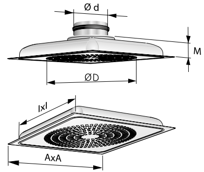
Figur 6. LOCKZONE Ceiling
