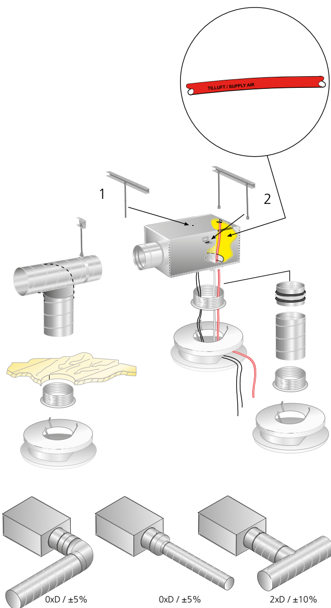
Figur 1. Montering. Injustering.
