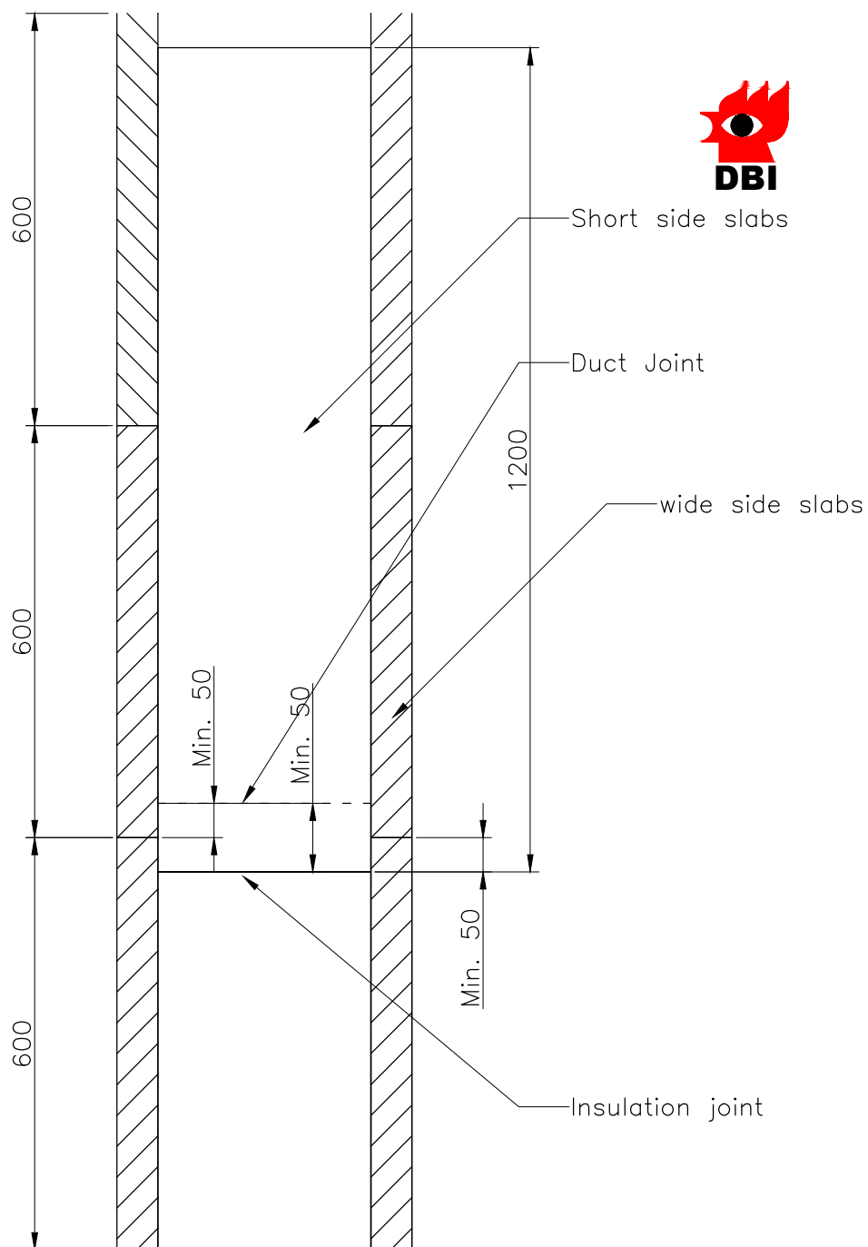
Minimum distance between slab joints
