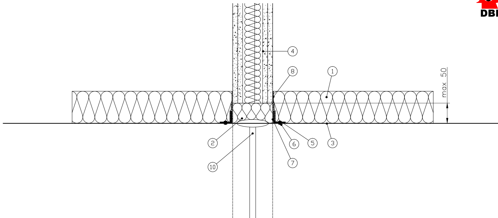
Detail of penetration through flexible wall
