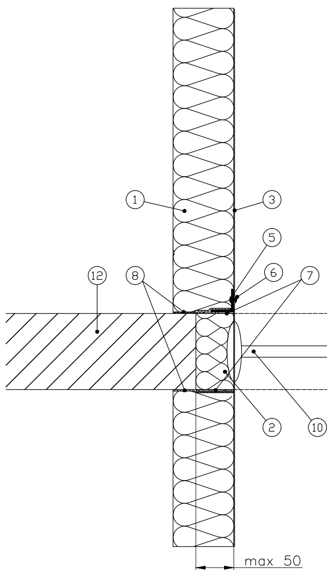
Detail of penetration through rigid floor
