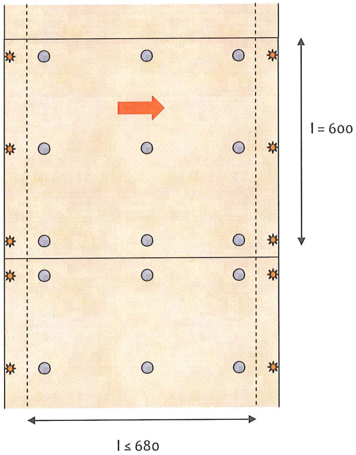
Slabs with overlapping
