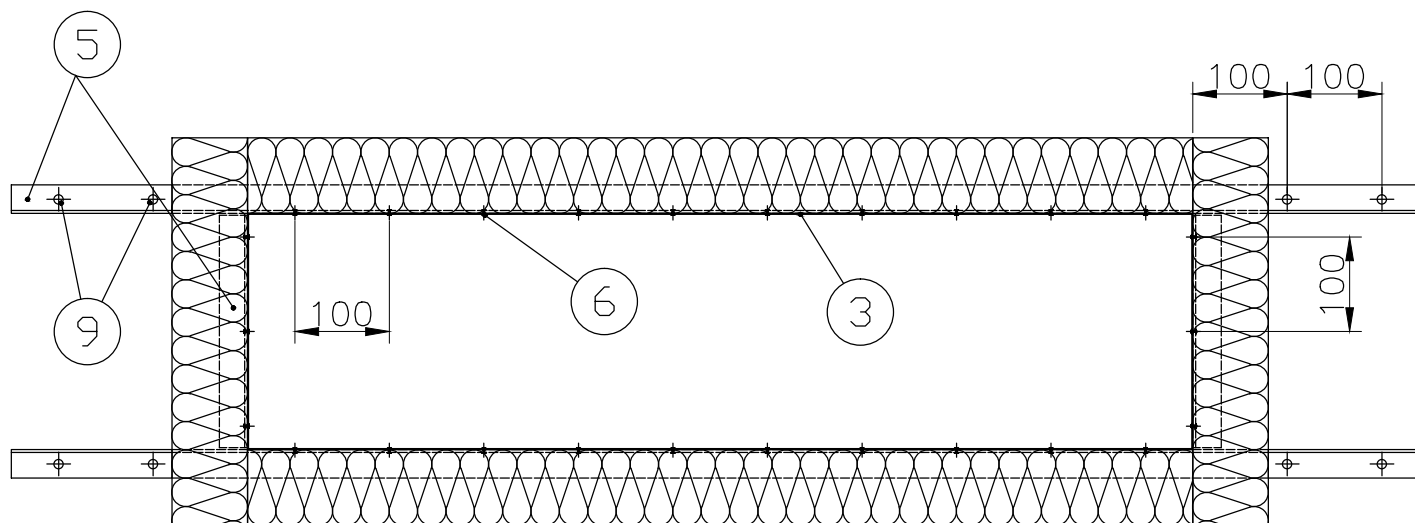
Fixing of duct to rigid wall or floor
