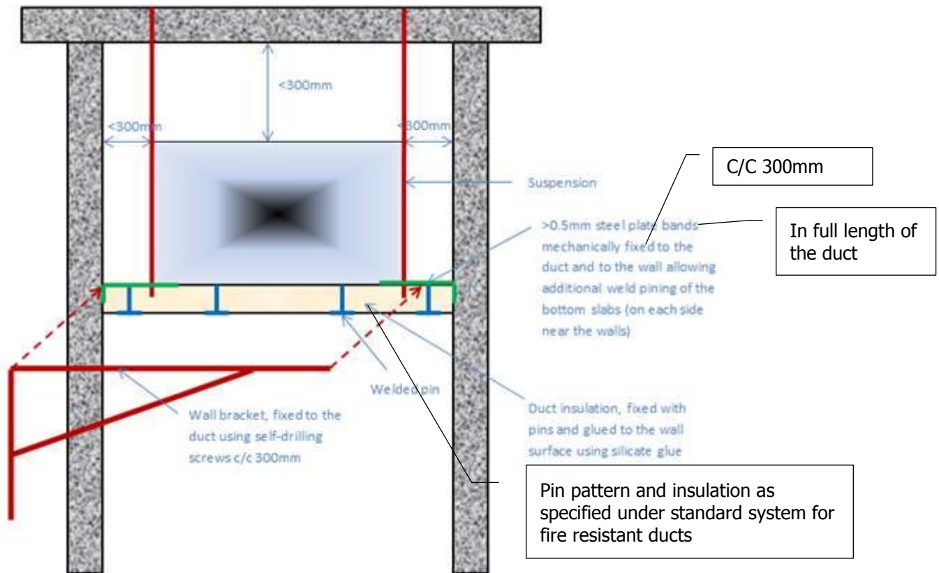
Front view of duct
