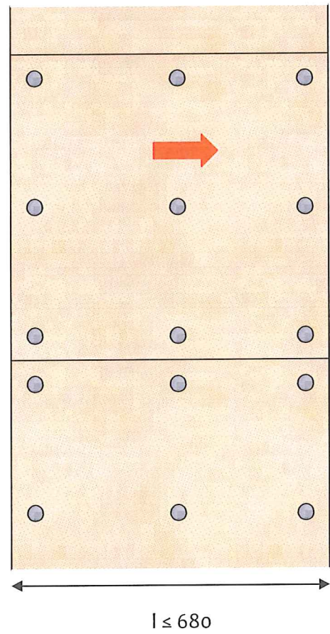
Slabs without overlapping
