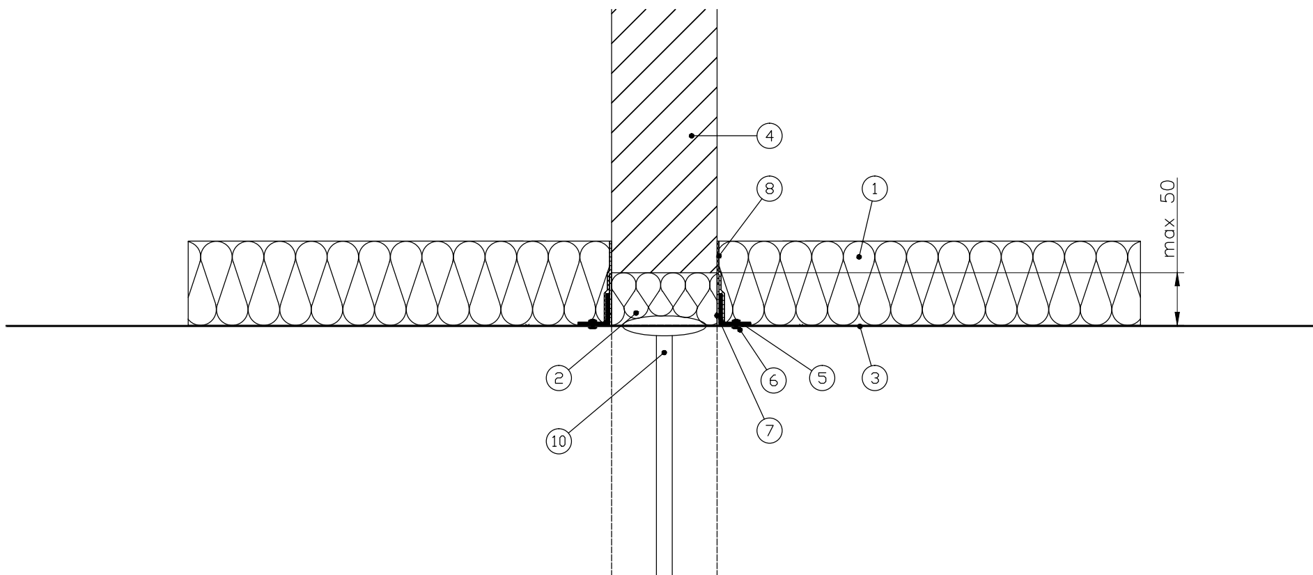
Detail of penetration through rigid wall
