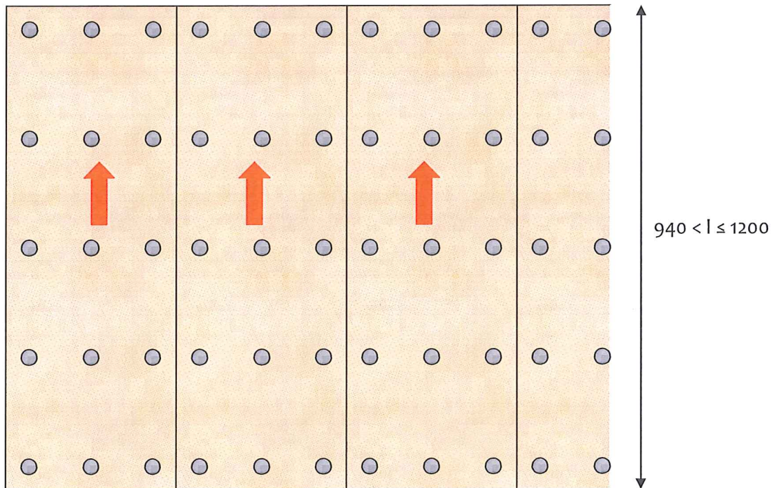
Side slabs
