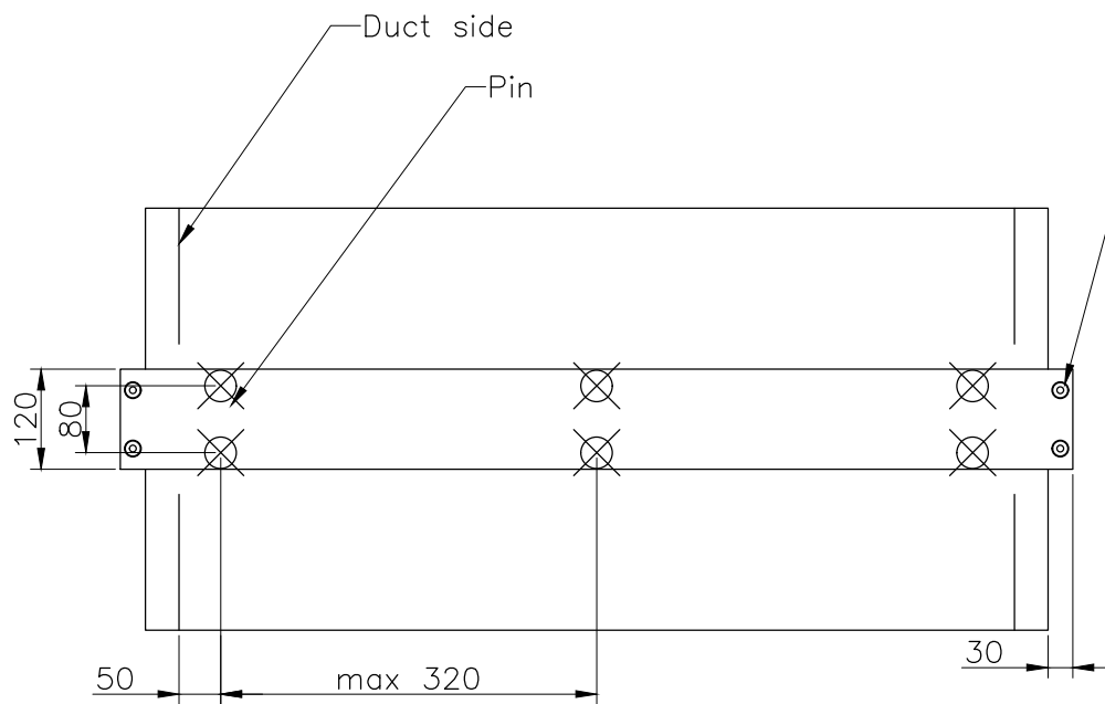
Wide side view
