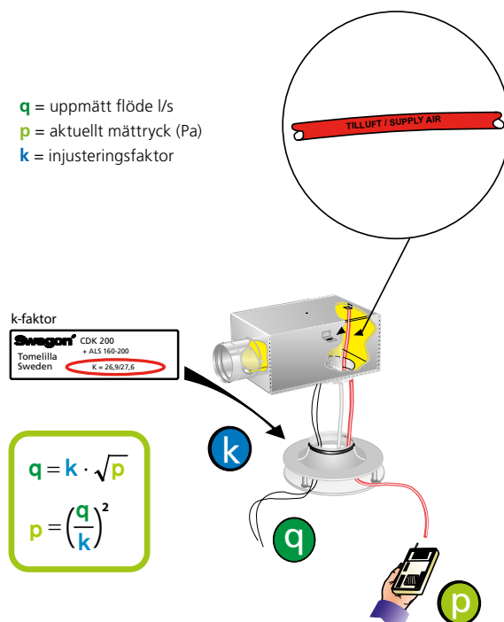
Figur 1. Injustering.
