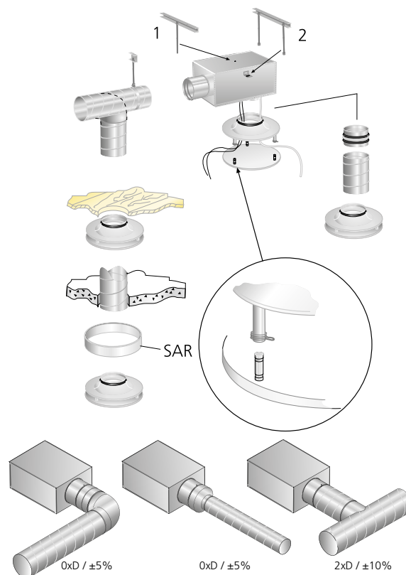
Figur 2. Montering.
