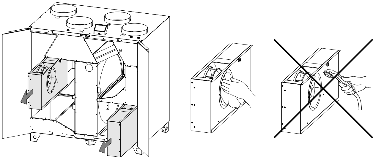
Fig. 7 Removing and cleaning the fans
