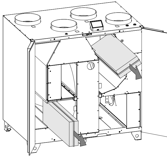
Fig. 5 Changing filters
