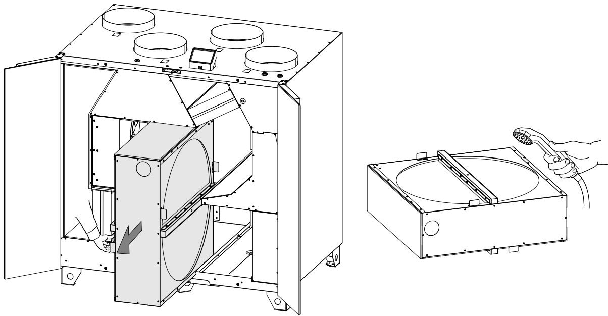
Fig. 6 Removing and cleaning the heat exchanger
