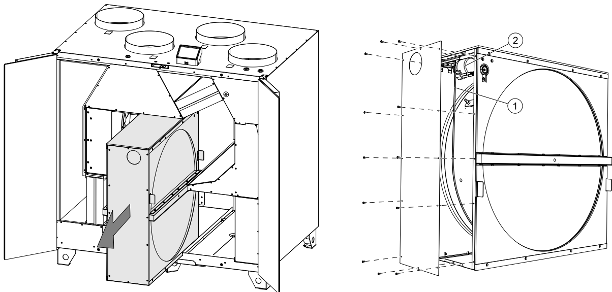
Fig. 8 Access broken rotor drive belt
