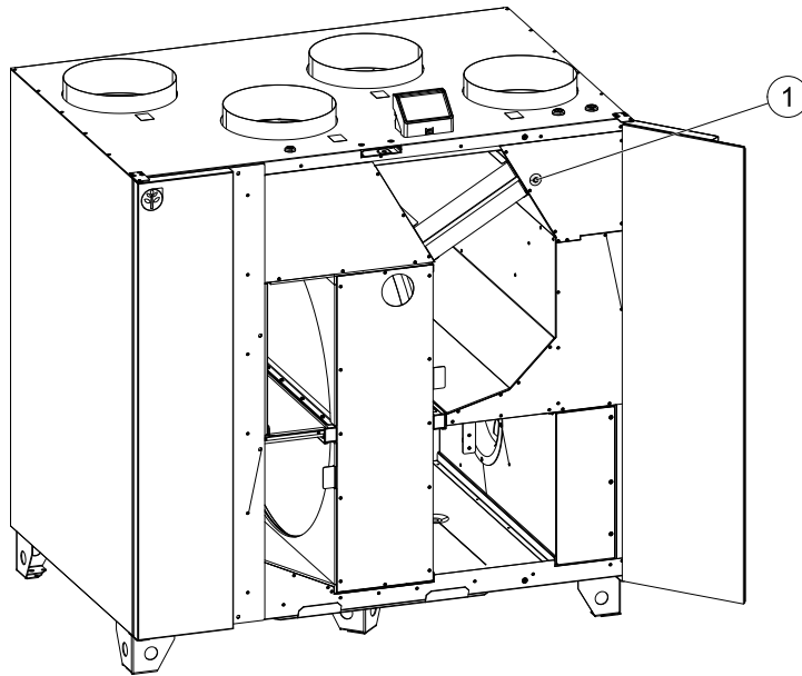
Fig. 9 Overheat protection reset button
