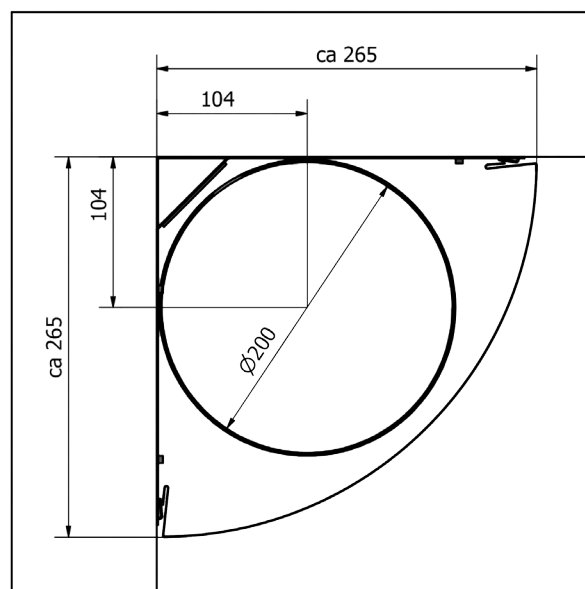
Ø200 under 200 panel
