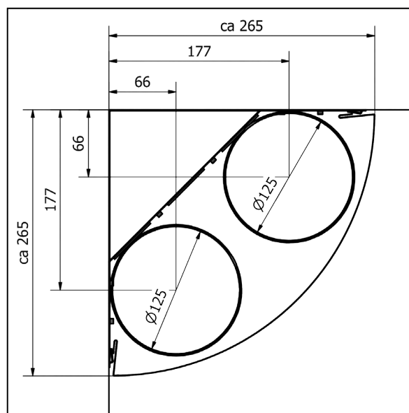
Ø125x2 under 200 panel
