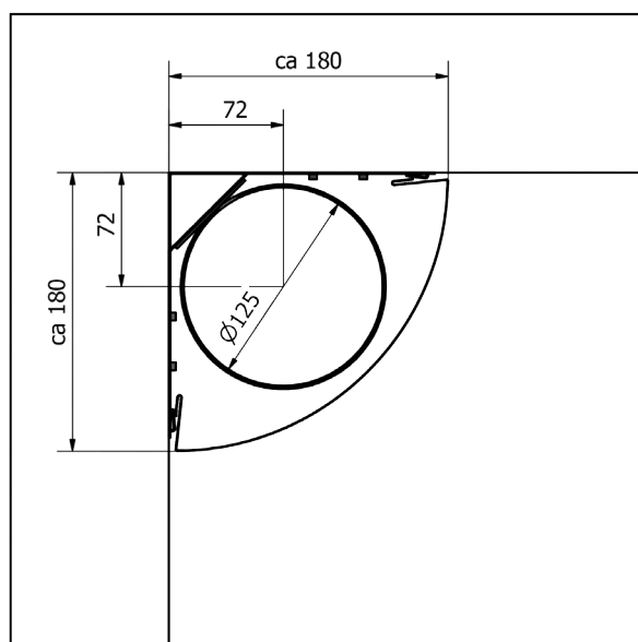
Ø125 under 125 panel
