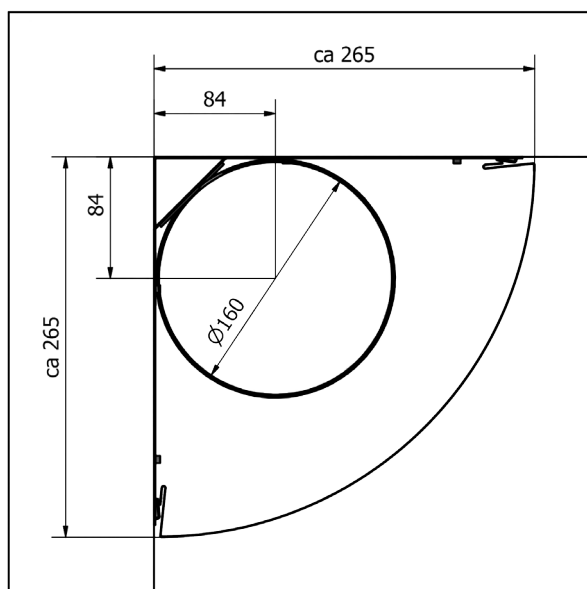
Ø160 under 200 panel
