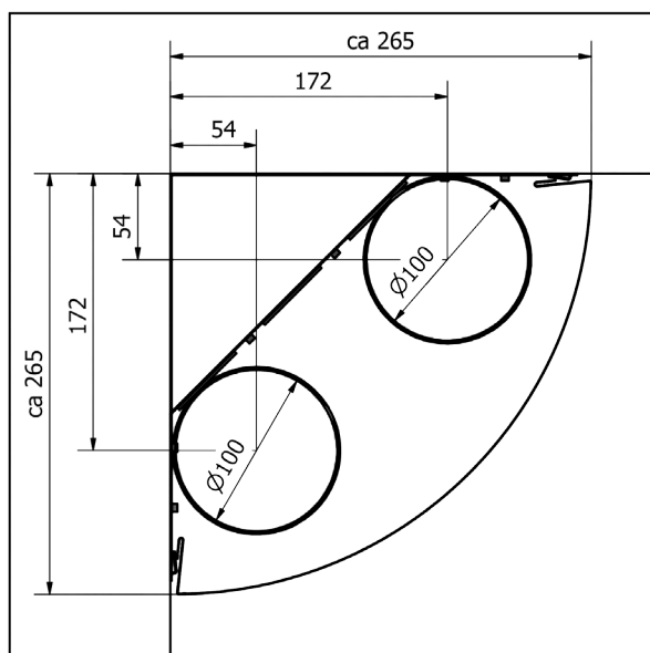
Ø100x2 under 200 panel
