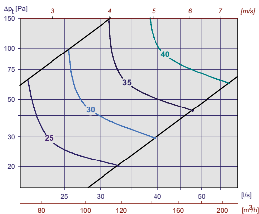
Diagram 3, TLG-LÖV m/Luna 100-160
