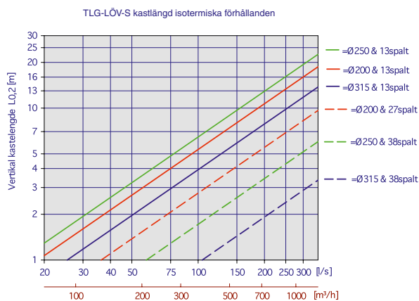
Diagram 19, Isoterm stål.
