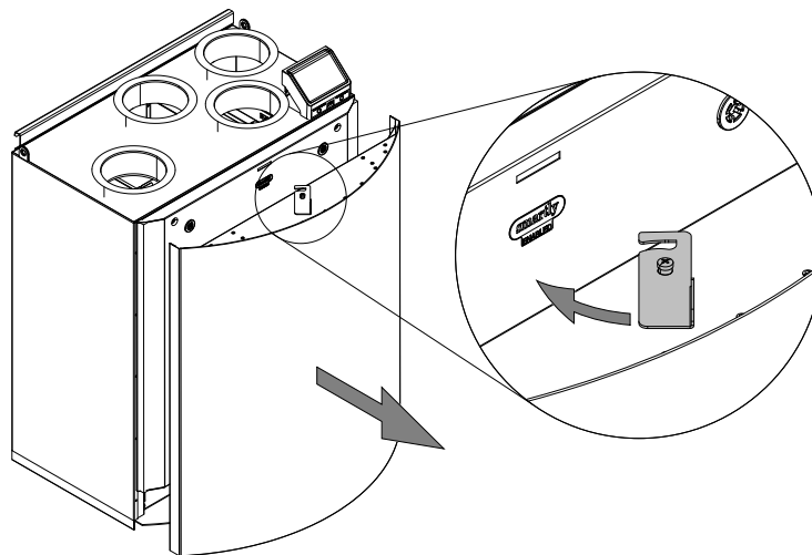
Fig. 5 Remove/mount the outer front
