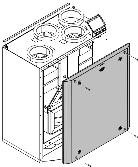
Fig. 6 Remove/mount the inner front
