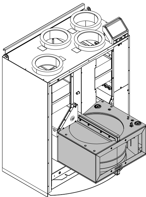
Fig. 8 Heat exchanger
