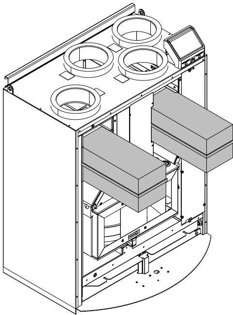
Fig. 7 Heat exchanger filters
