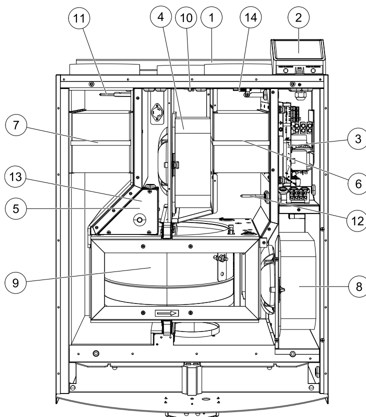
Fig. 12 Internal components
