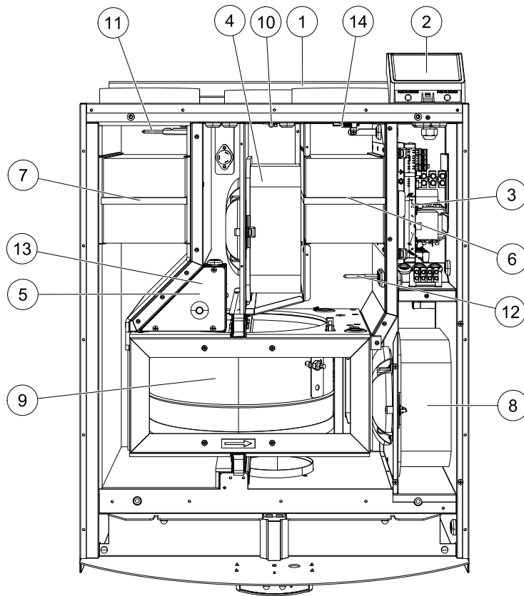
Fig. 12 Internal components
