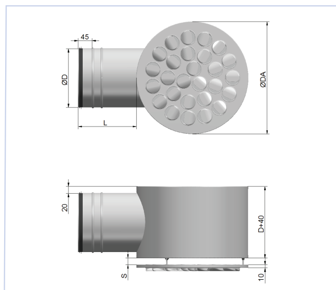
Figur 1, Tellus-Opus-L
