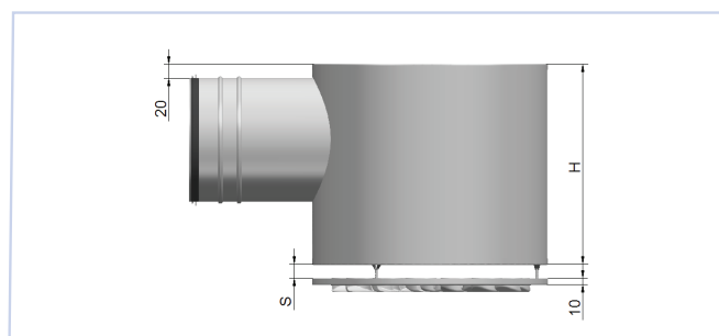
Figur 2, Tellus-Opus-H
